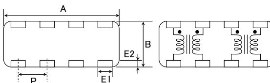
Equivalent Circuit •No polarity
