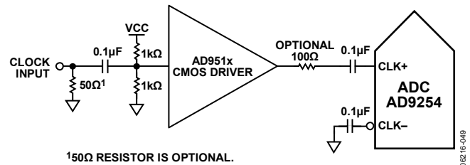
150Ω RESISTOR IS OPTIONAL. Figure 45. Single-Ended 3.3 V CMOS Sample Clock
