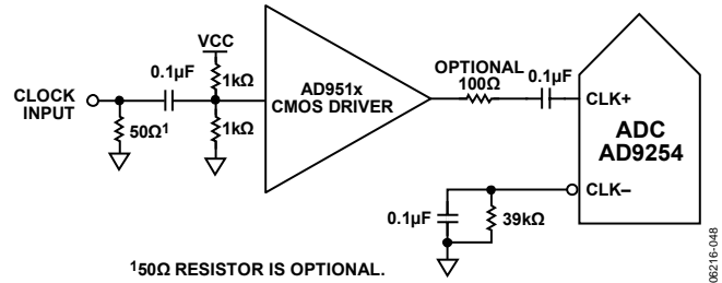
150Ω RESISTOR IS OPTIONAL. Figure 44. Single-Ended 1.8 V CMOS Sample Clock
