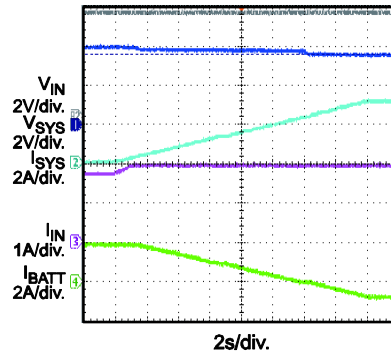
Input Voltage Limit 5V/1A \text{ Adapter IN} , V_{BATT} = 4.2V Ramp up I_{SYS}
