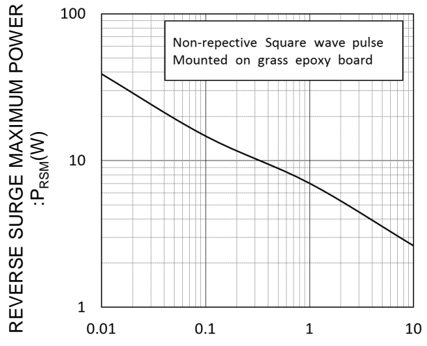
P_{RSM}-t CHARACTERISTICS
