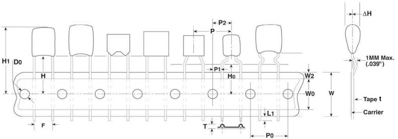
Figure 3: Standard Reel
