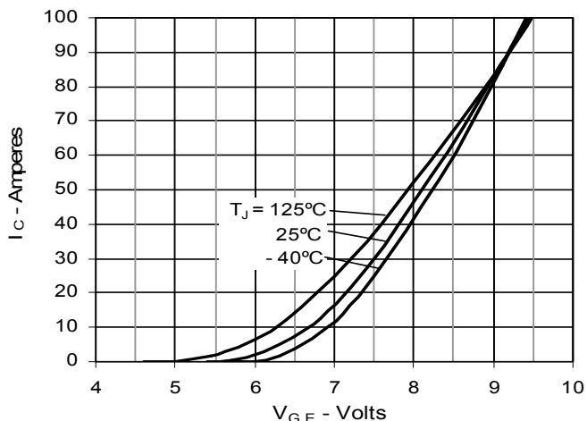
Fig. 6. Input Admittance
