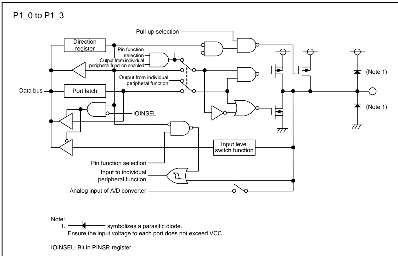
Figure 7.3 Configuration of I/O Ports (3)
