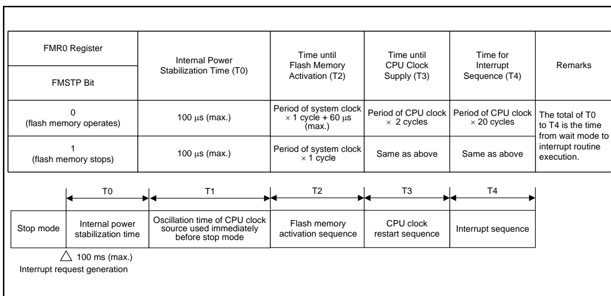
Figure 9.6 Time from Stop Mode to Interrupt Routine Execution
