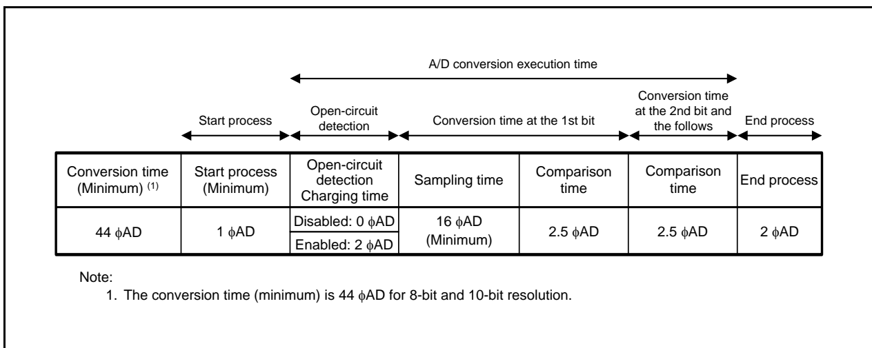
Figure 25.3 A/D Conversion Cycles ( \phi_{AD} = f_{AD} )
