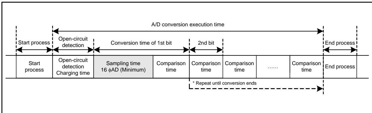
Figure 25.2 Timing Diagram of A/D Conversion
