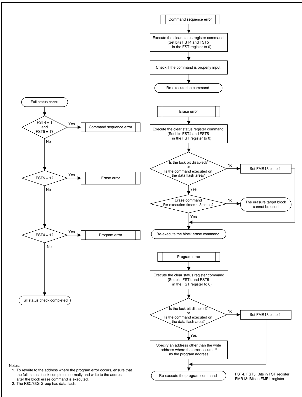
Figure 28.16 Full Status Check and Handling Procedure for Individual Errors
