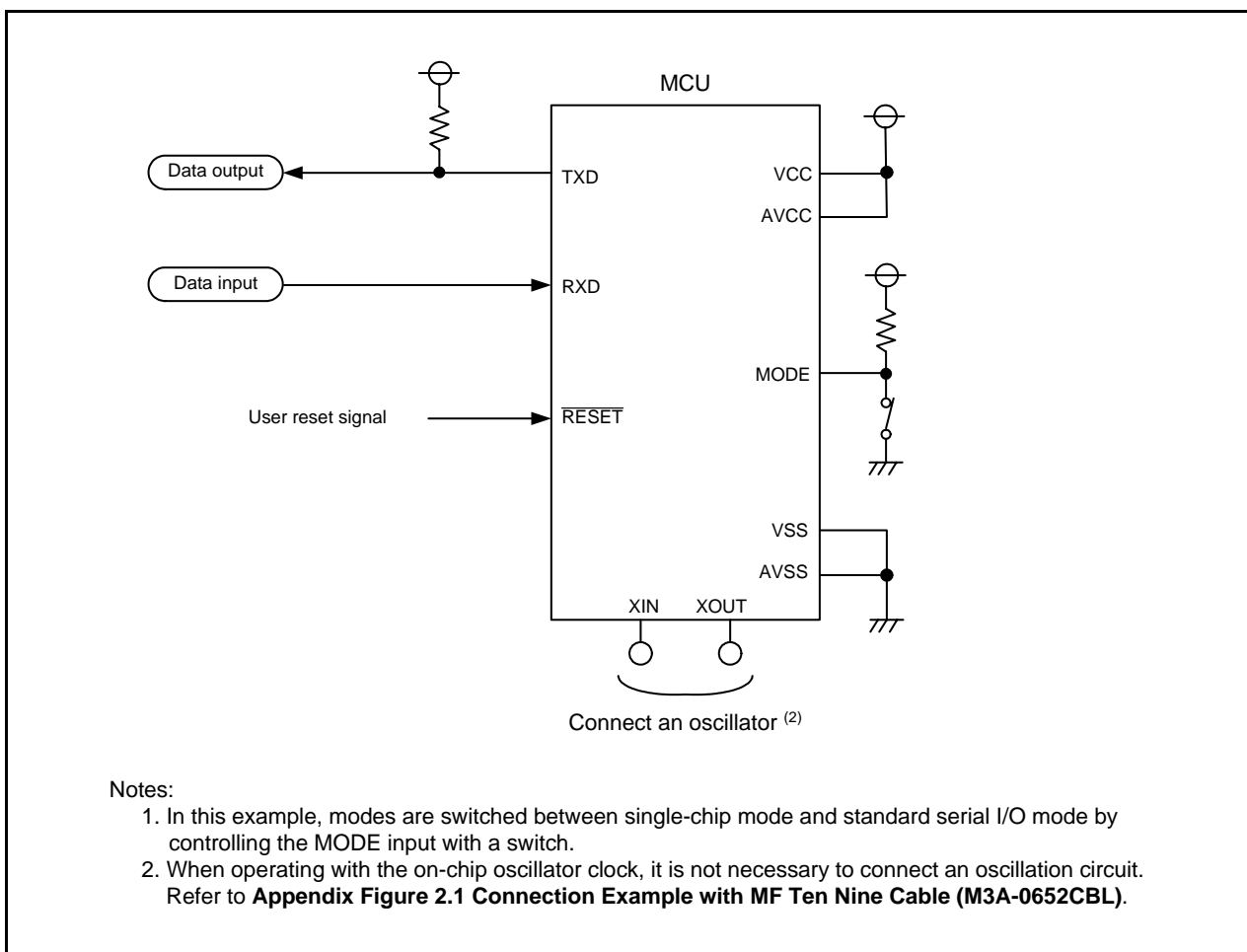
Figure 28.17 Pin Handling in Standard Serial I/O Mode 2
