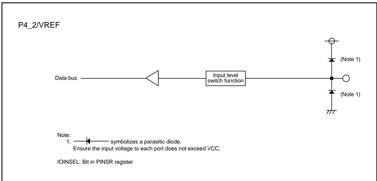
Figure 7.9 Configuration of I/O Ports (9)
