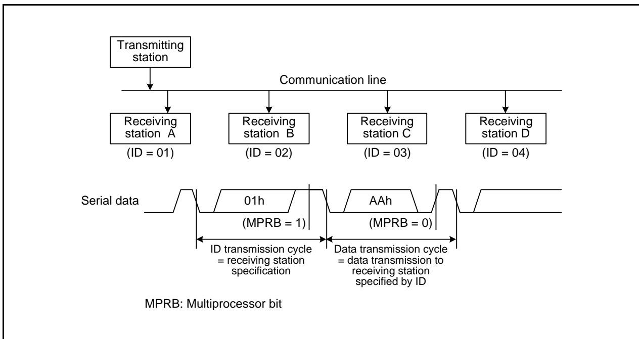
Figure 22.18 Inter-Processor Communication Example Using Multiprocessor Format (Data AAh Transmission to Receiving Station A)
