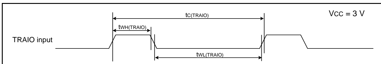
Figure 30.12 TRAIO Input Timing Diagram when V_{CC} = 3\text{ V}
