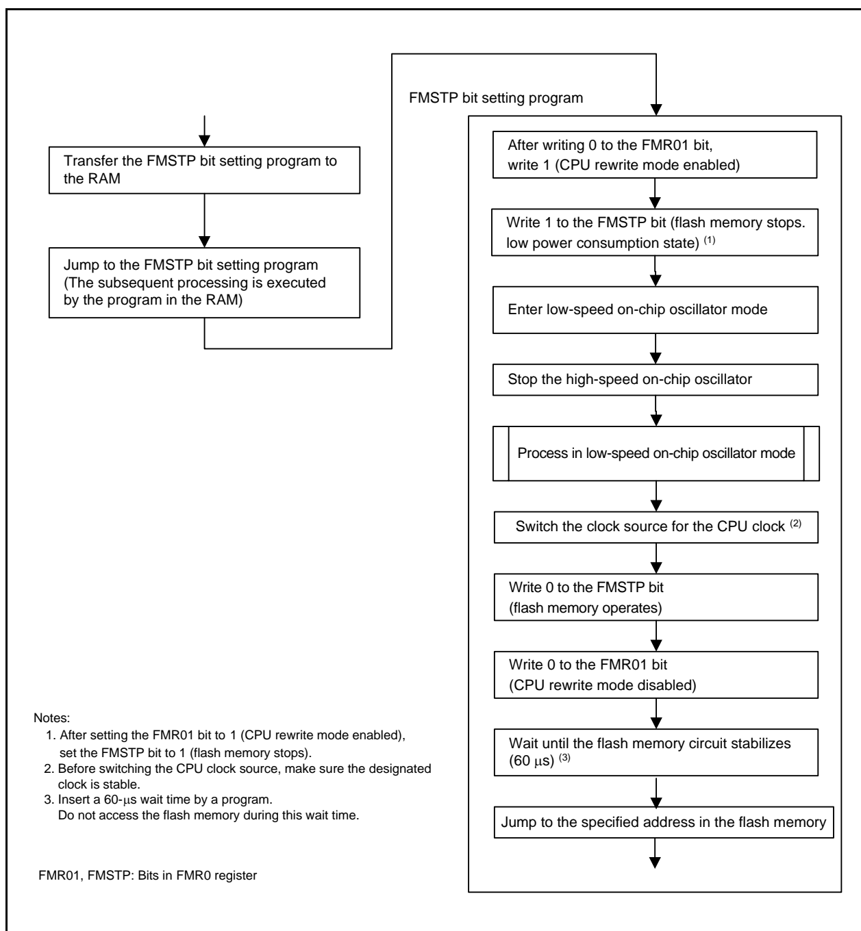
Figure 29.3 Handling Procedure Example for Reducing Power Consumption Using FMSTP Bit
