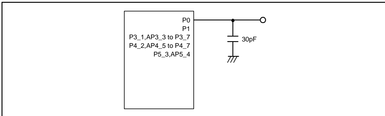
Figure 30.1 Ports P0 to P1, P3_1, P3_3 to P3_7, P4_2, P4_5 to P4_7, P5_3, and P5_4 Timing Measurement Circuit
