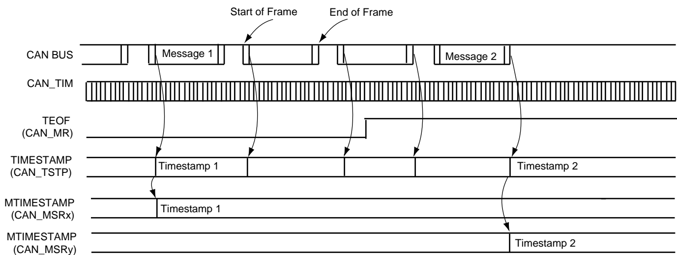
Figure 32-19. Mailbox Timestamp
