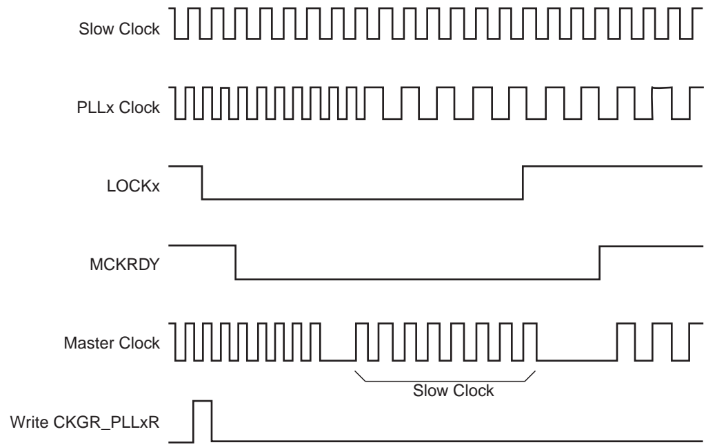
Figure 30-11. Change PLLx Programming
