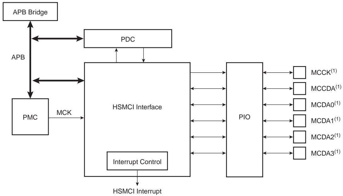
Figure 39-1. Block Diagram
