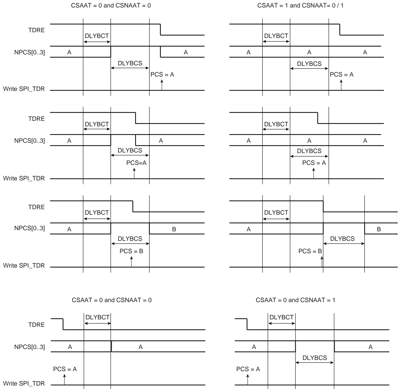
Figure 34-12. Peripheral Deselection
