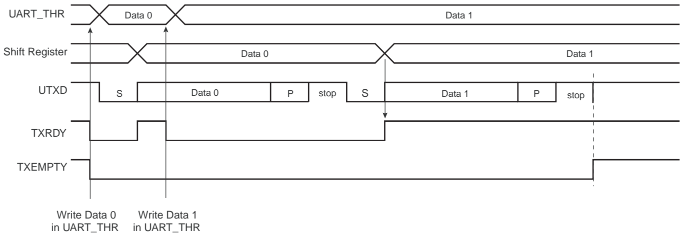
Figure 36-10. Transmitter Control
