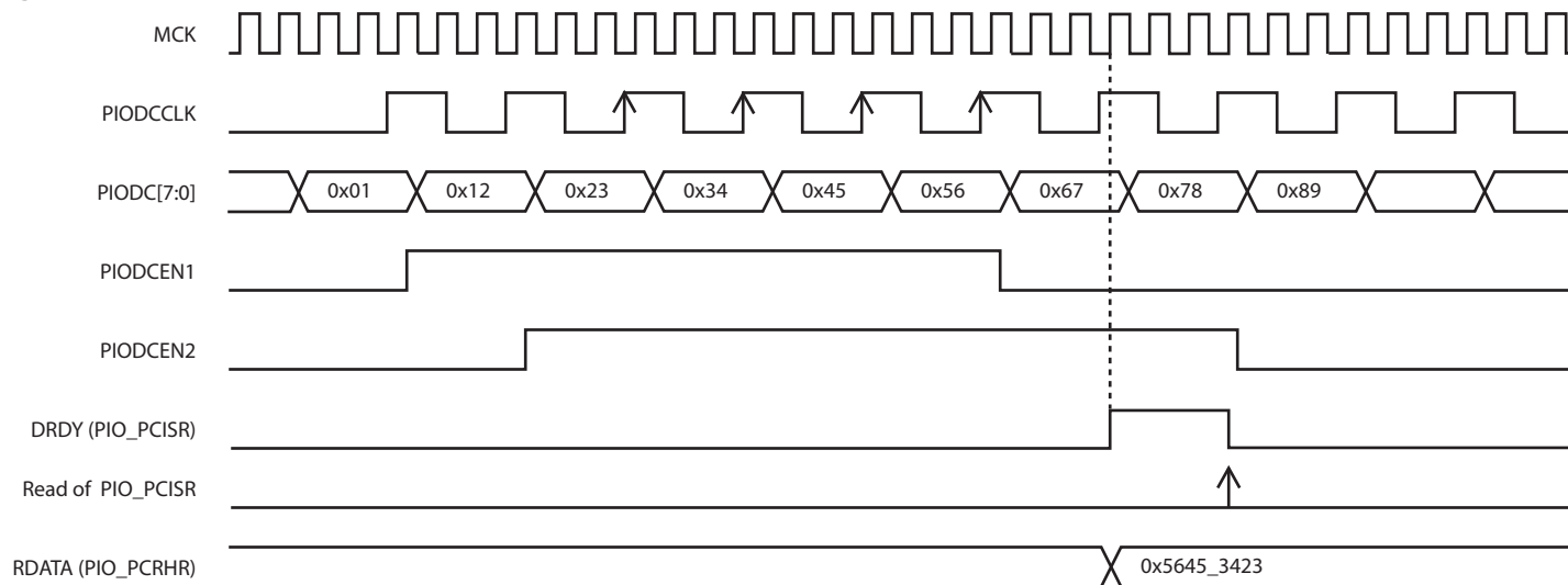
Figure 33-12. Parallel Capture Mode Waveforms (DSIZE = 2, ALWAYS = 0, HALFS = 0)
