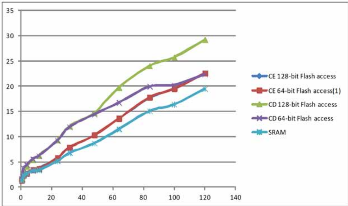
Figure 46-10. Active Total Power Consumption with VDDCORE @ 1.2V
