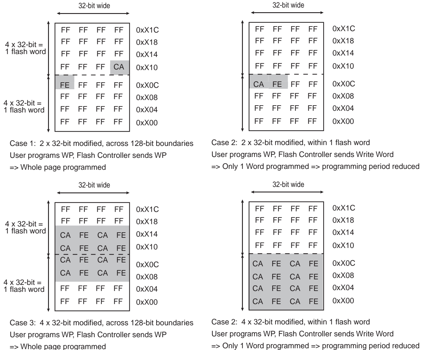
Figure 22-8. Optimized Partial Programming
