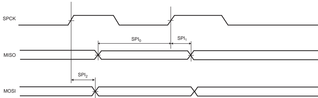
Figure 46-16. SPI Master Mode with (CPOL= NCPHA = 0) or (CPOL= NCPHA= 1)
