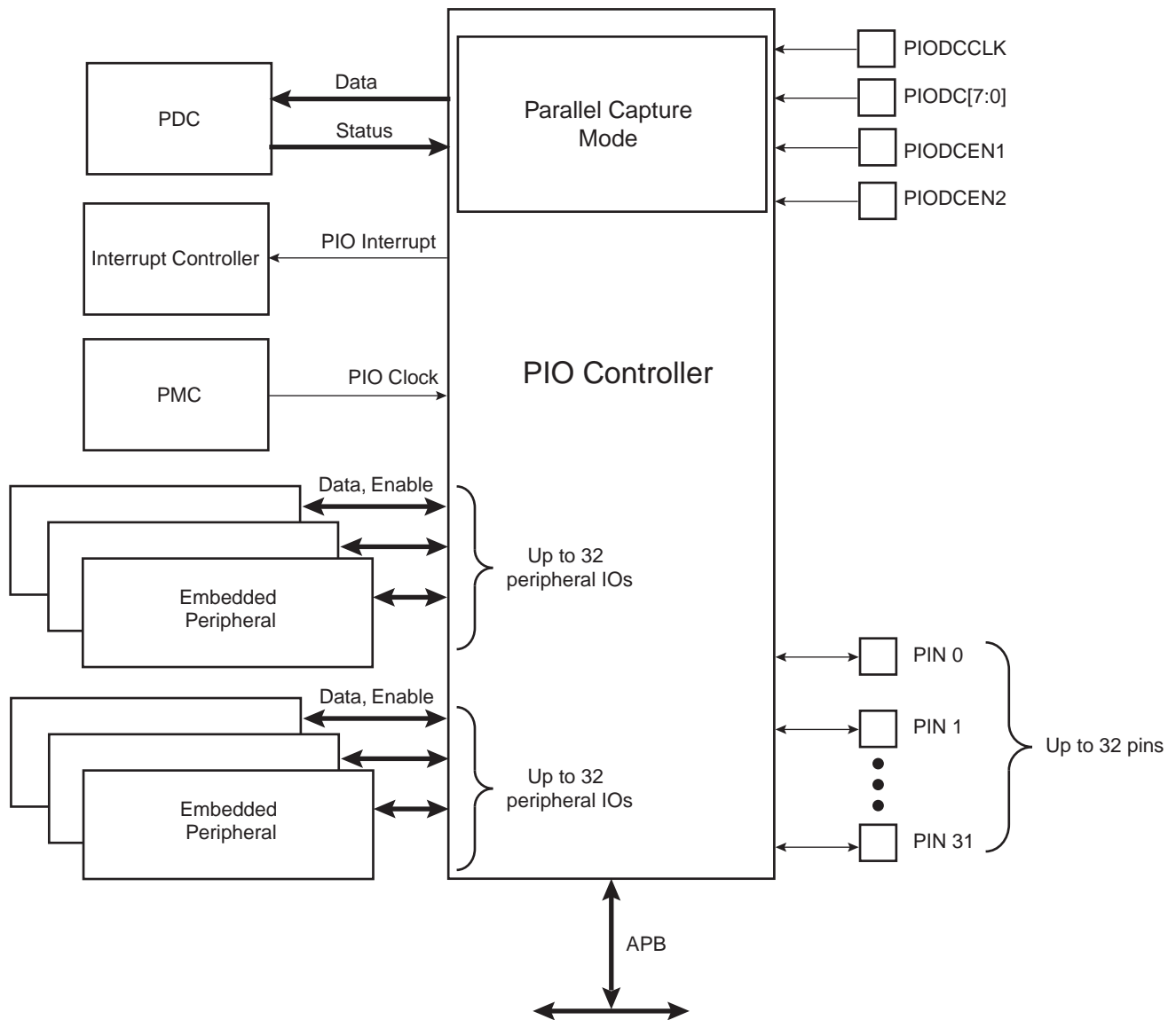
Figure 33-1. Block Diagram
