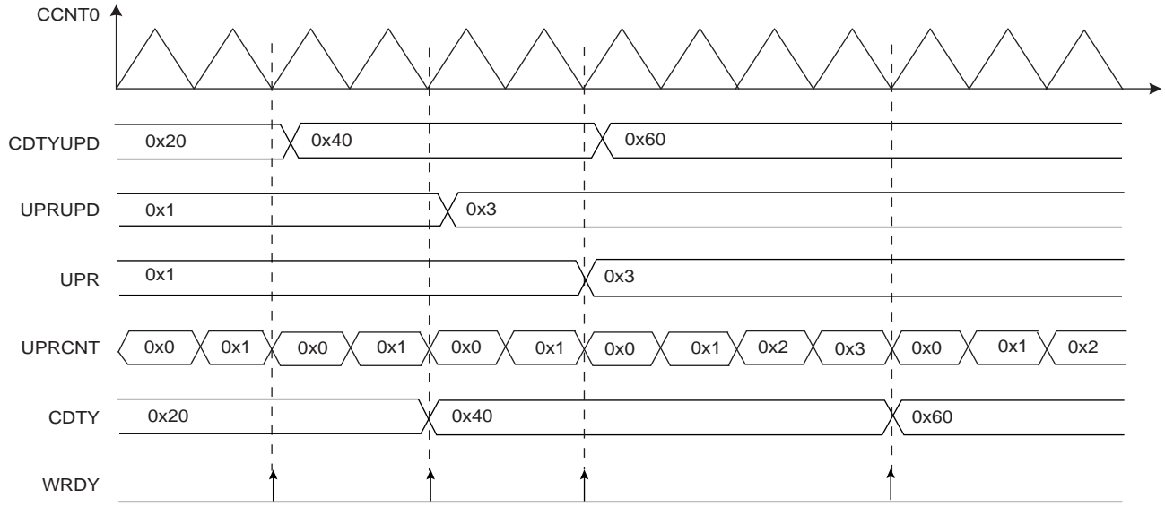
Figure 40-13. Method 2 (UPDM=1)
