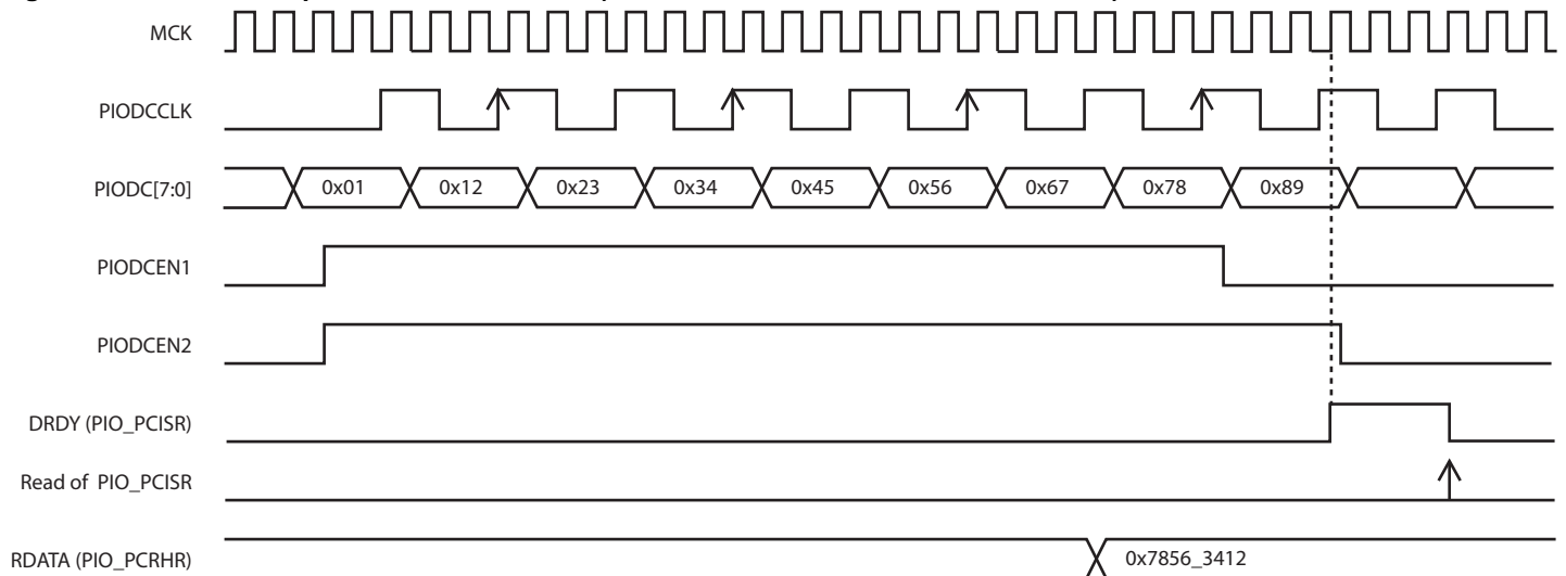
Figure 33-15. Parallel Capture Mode Waveforms (DSIZE=2, ALWAYS=0, HALFS=1, FRSTS=1)
