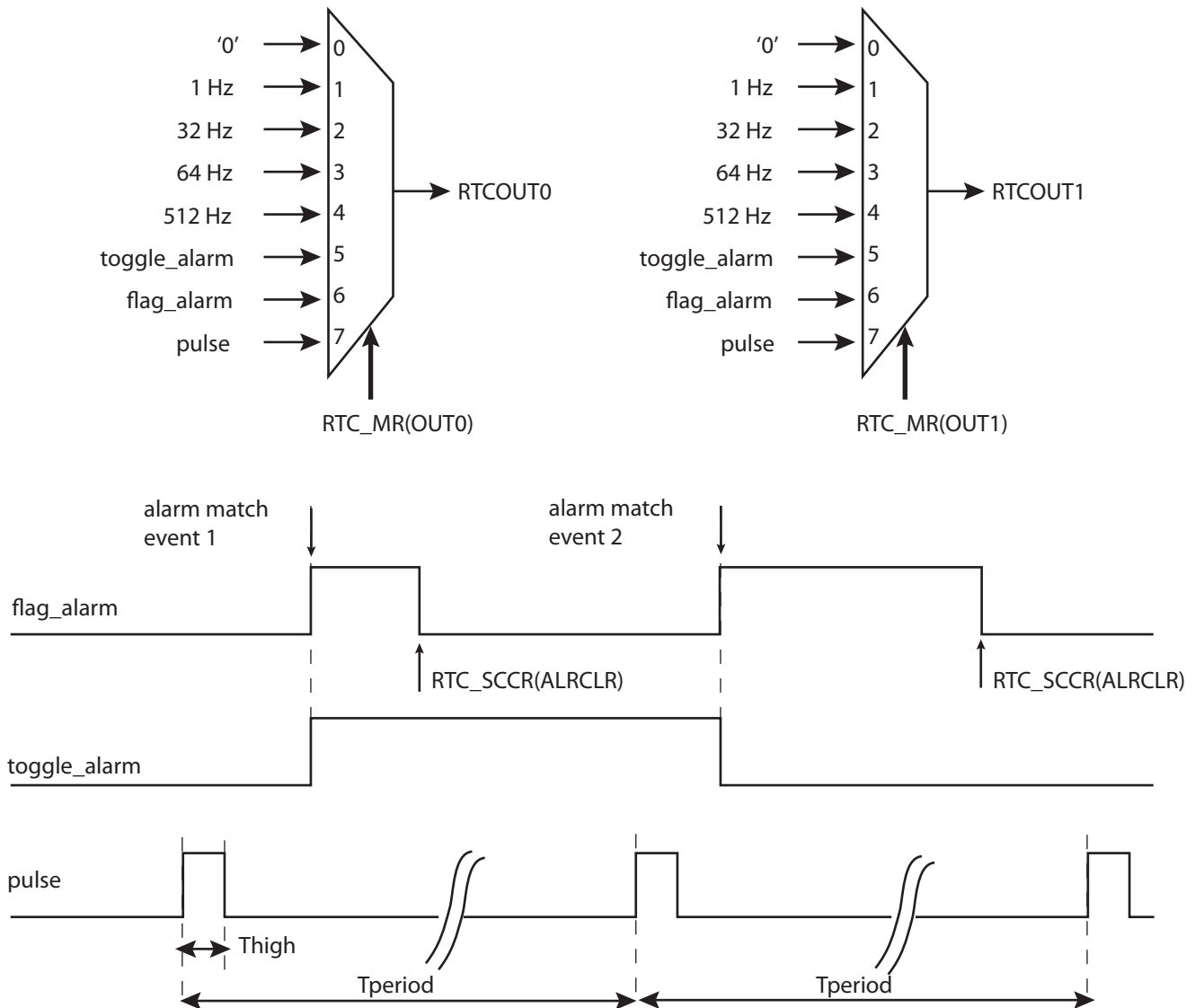
Figure 18-3. Waveform Generation
