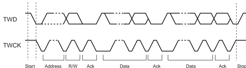
Figure 35-4. Transfer Format
