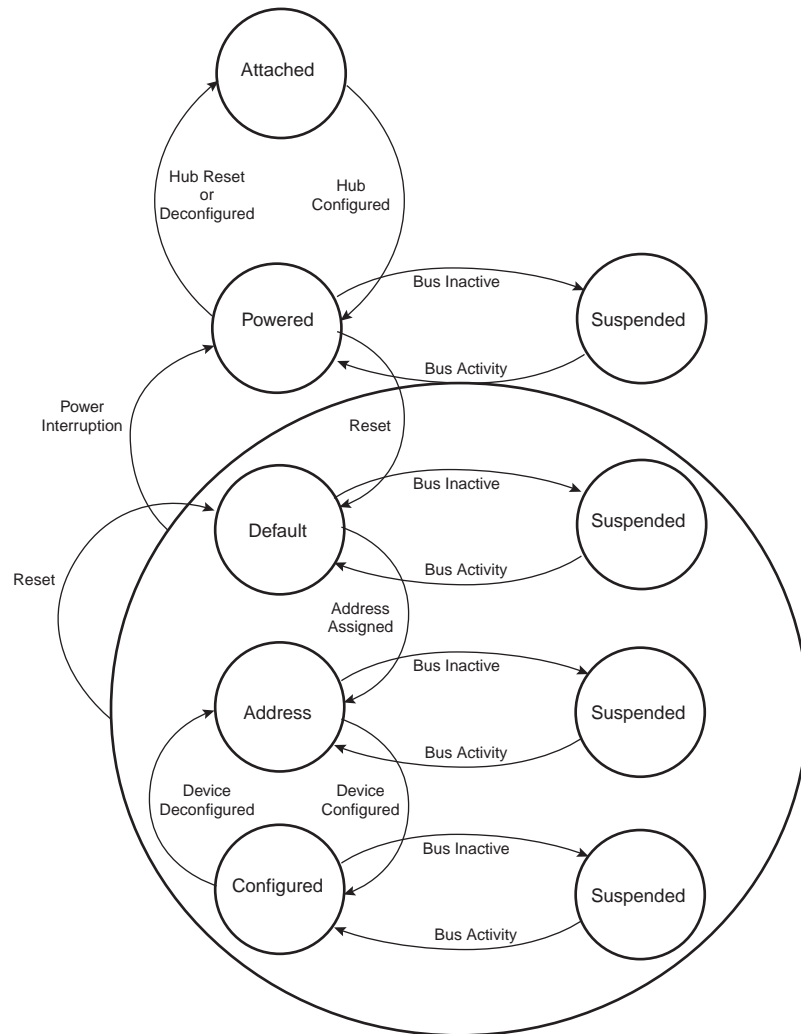
Figure 41-14. USB Device State Diagram
