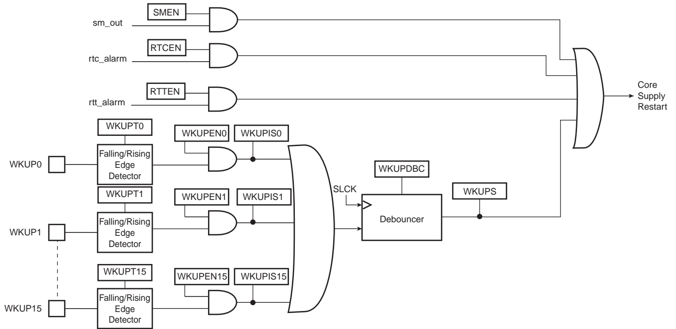
Figure 5-3. Wake-up Source
