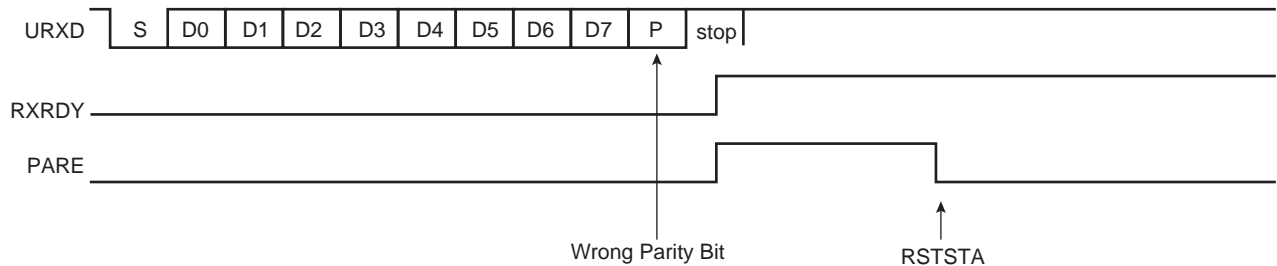
Figure 36-7. Parity Error
