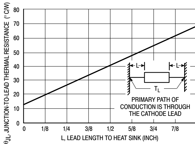
Figure 9. Typical Thermal Resistance
