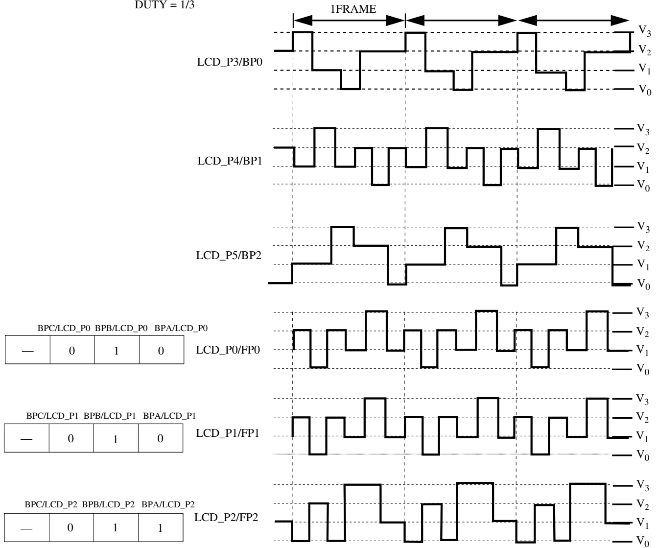
Figure 52-40. LCD waveforms
