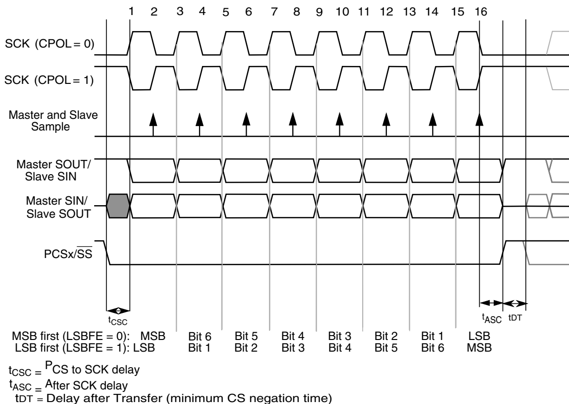
Figure 45-95. DSPI Transfer Timing Diagram (MTFE=0, CPHA=1, FMSZ=8)
