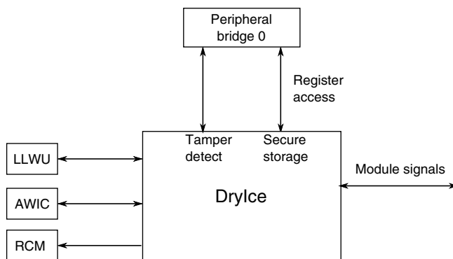
Figure 3-31. Drylce configuration
