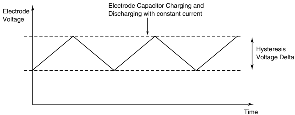
Figure 51-65. TSI electrode oscillator chart
