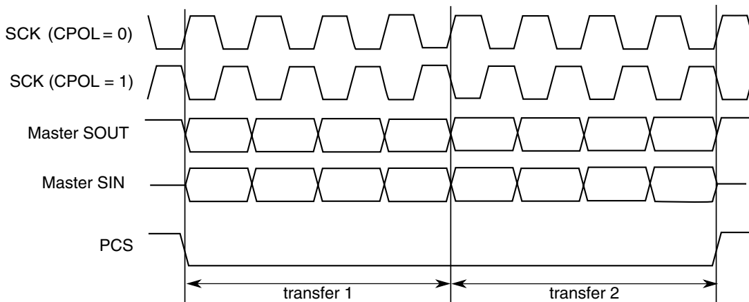
Figure 45-99. Continuous SCK Timing Diagram (CONT=1)
