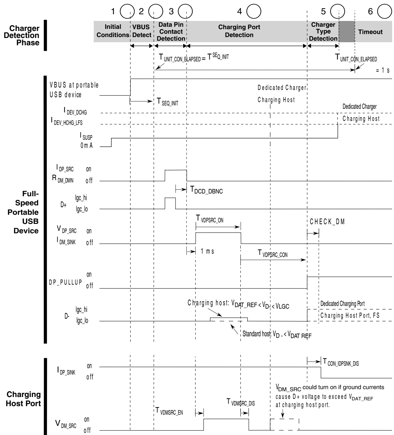
Figure 42-9. Full Speed Charger Detection Timing
