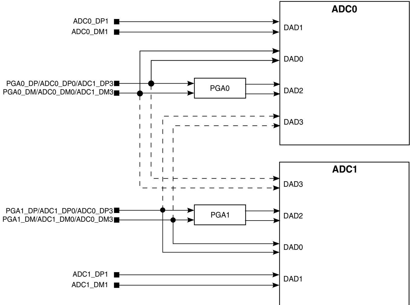
Figure 3-35. PGA Integration
