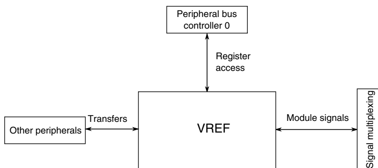
Figure 3-38. VREF configuration
