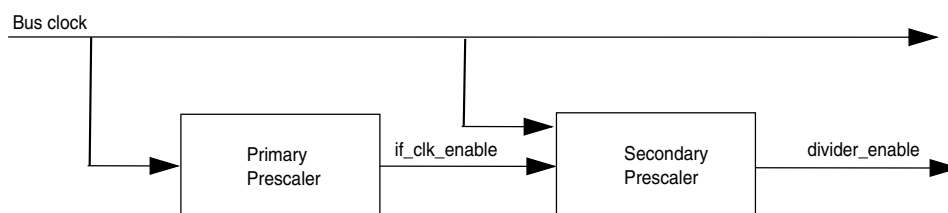
Figure 39-14. Clock Divider Block Diagram
